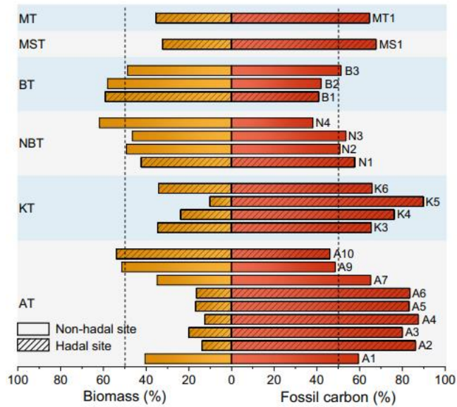
Figure 8. Radioactive carbon isotopic composition ( \Delta^{14}\text{C} )-based estimate for proportion (%) of fossil carbon and biomass burning to the Black carbon pool in surface sediments from six trench regions (Zhang et al., 2022).
