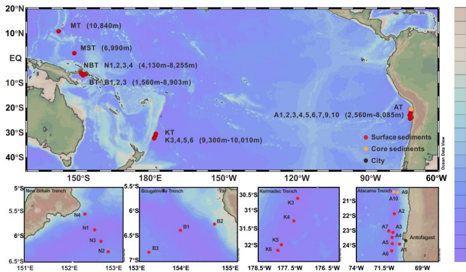
Figure 7. The distribution and concentration of black carbon were studies in six hadal trenches around the world (Zhang et al., 2022).
